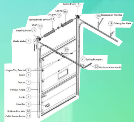
EXPLODED VIEW
